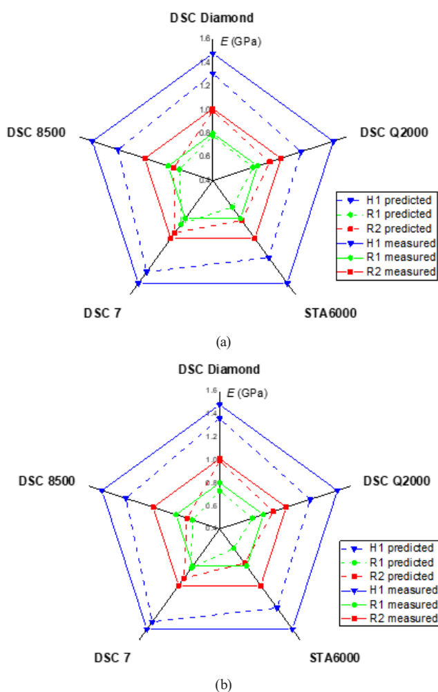
Fig. 8 Visual representation of instrument dependency of the modulus estimations based on logistic function (a), and exponential function (b)
