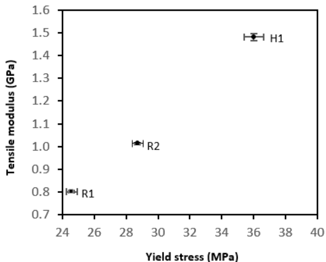
Fig. 6 Modulus as a function of yield stress for used materials
