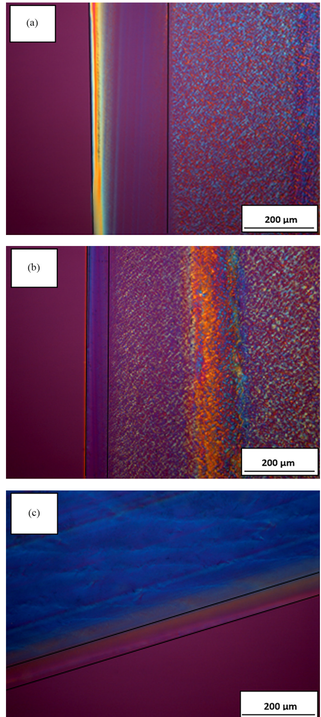
Fig. 3 PLM images of samples – (a) H1, (b) R1, (c) R2
