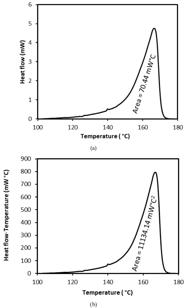
Fig. 1 Heat flow curve (a), Heat flow · Temperature curve (b)
