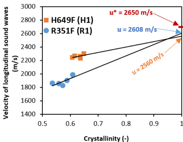
Fig. 2 Propagation velocity of sound waves as a function of crystallinity ( R_{R1}^2 = 0.86 ; R_{H1}^2 = 0.73 ). * Propagation velocity of longitudinal sound waves ( u ) for perfectly crystalline polymer ( X = 1 ) according to van Krevelen and te Nijenhuis [38]
