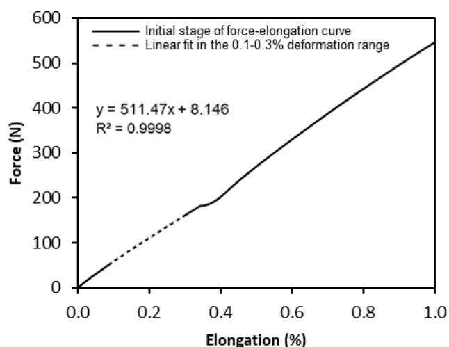
Fig. 5 Evaluation of slope of the force-elongation curve
